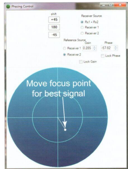
Fig. 5: PowerSDRmRx phase adjustment panel for diversity reception.
