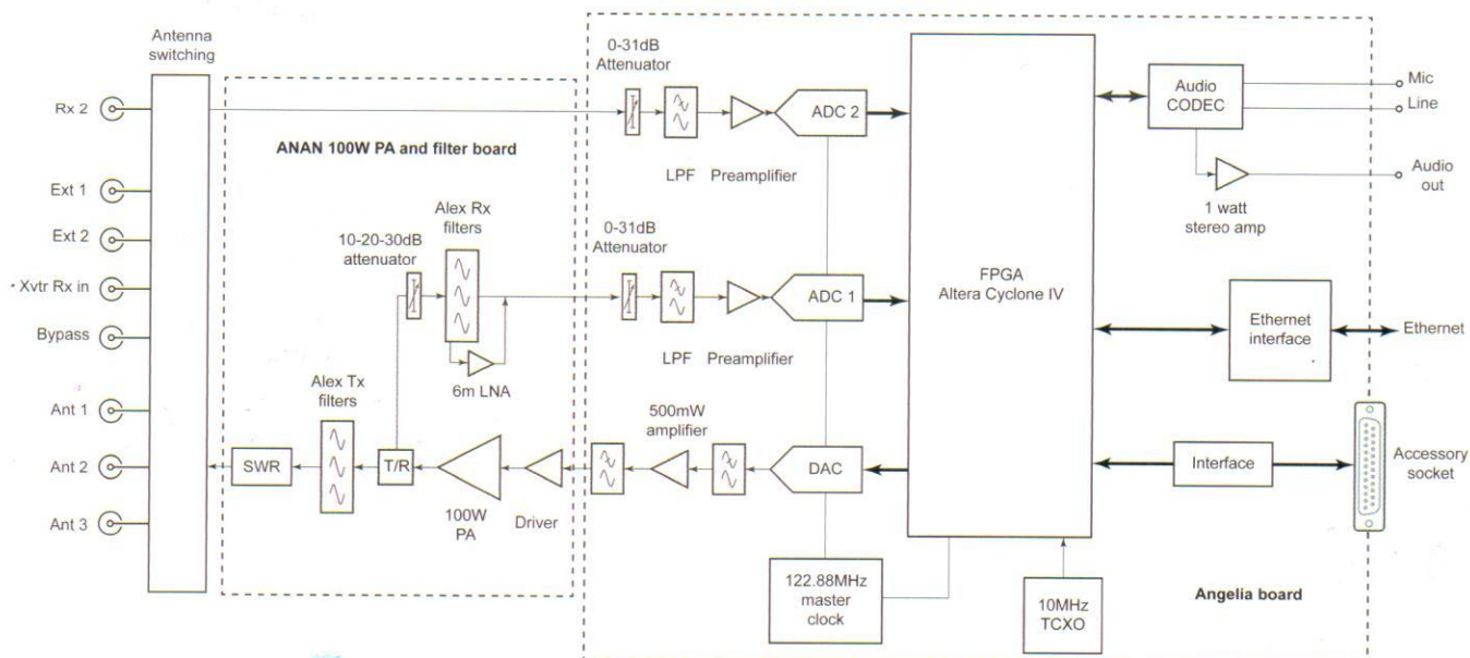
Fig. 1. Simplified block diagram of the ANAN-100D.
