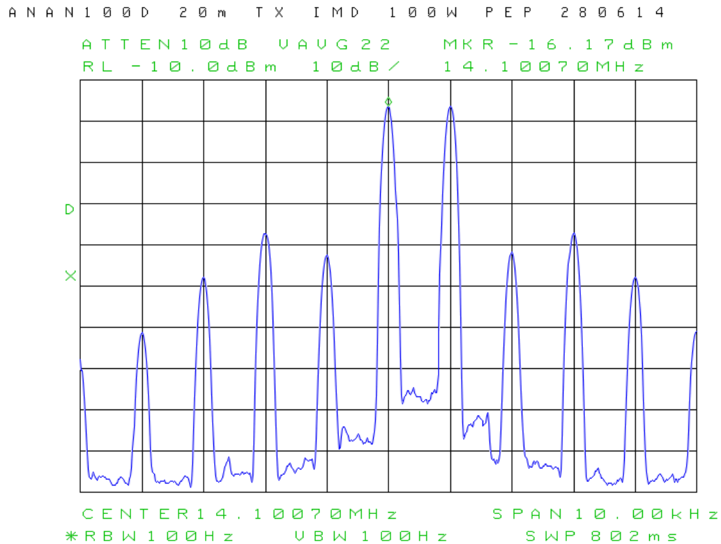
Figure 13: Spectral display of 2-tone IMD at 14.1 MHz, 100W PEP.
