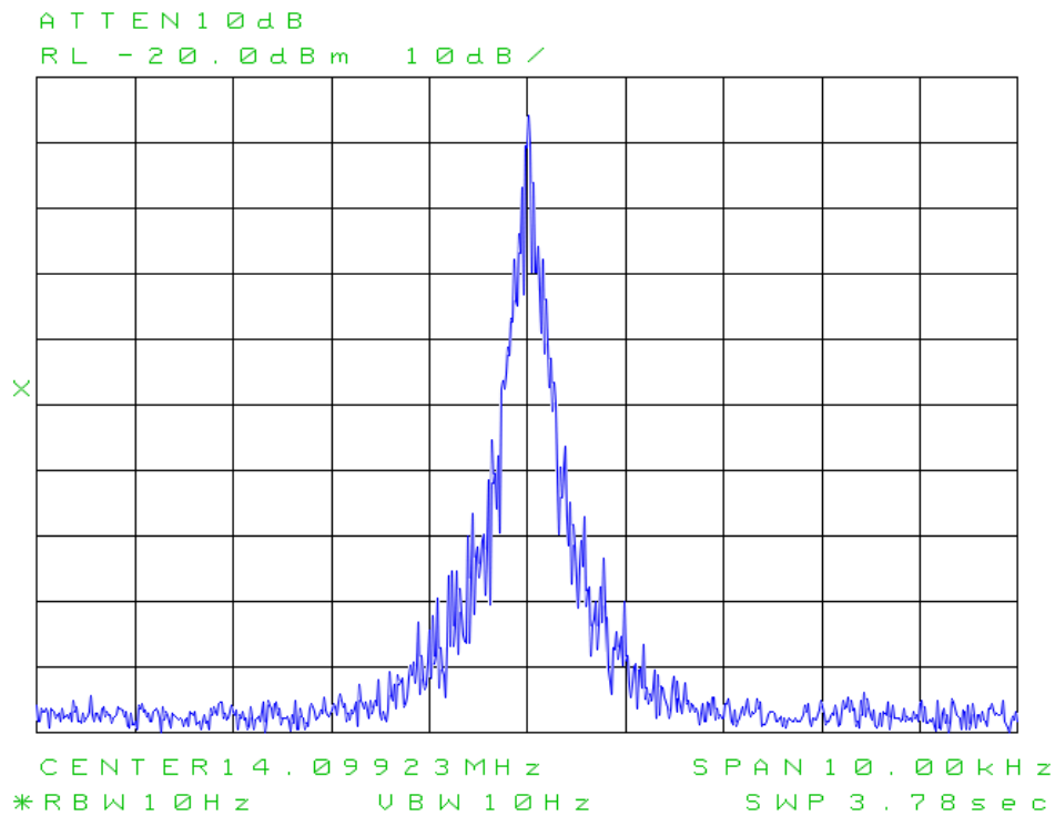
Figure 21: Keying sidebands at 60 wpm, Weight = 50%, 14.1 MHz, 50W.
