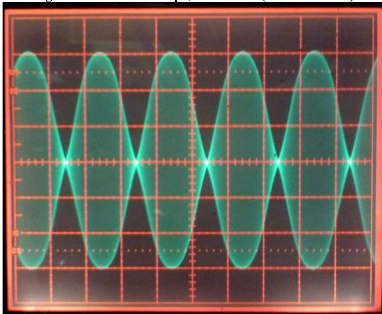
Figure 11: 2-tone envelope, 100W PEP ( = \pm 3 vert. div.)
