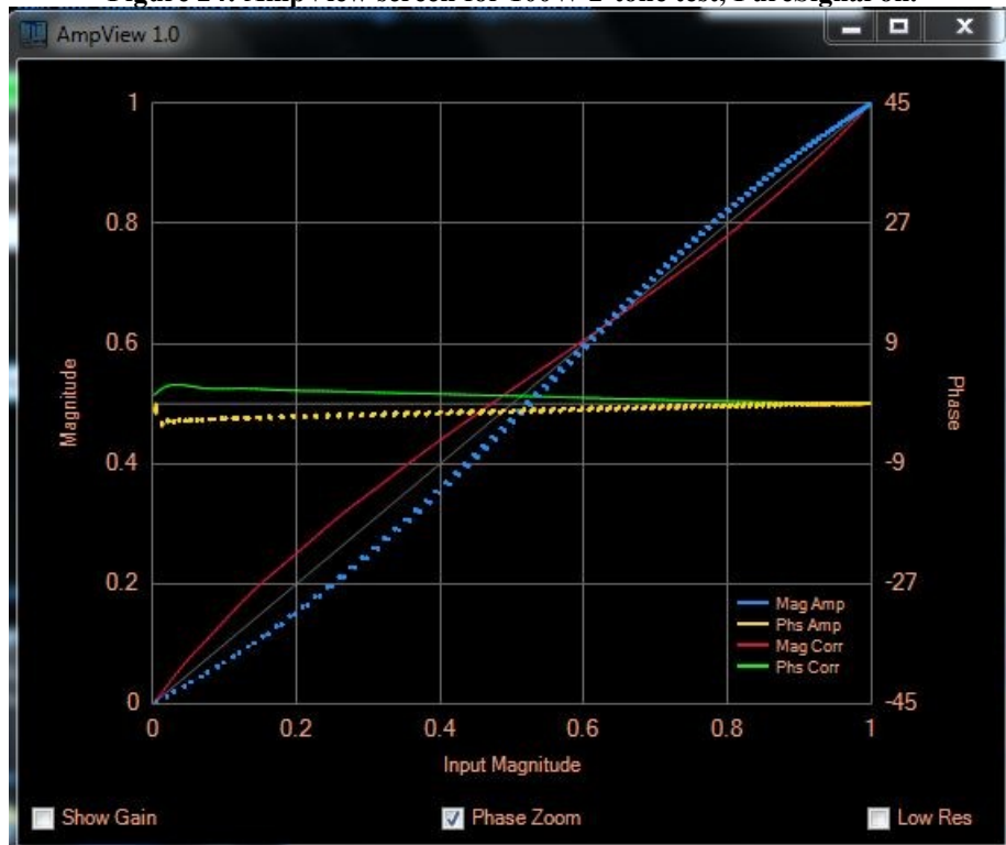
Figure 24: AmpView screen for 100W 2-tone test, PureSignal on.
