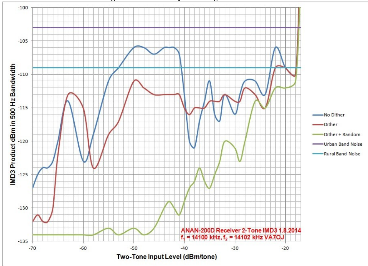
Figure 1: 2-tone IMD_3 vs. test signal level.
