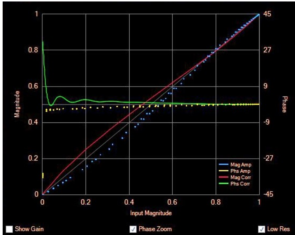
Figure 3: AmpView screen for 100W 2-tone test, PureSignal on (Test 9).
