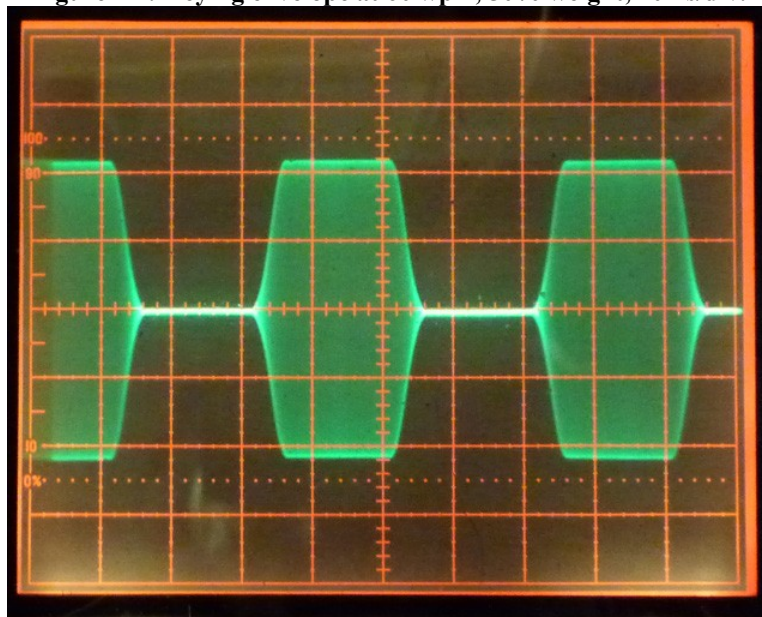
Figure 22: Keying envelope at 60 wpm, 50% weight, 10ms/div.
