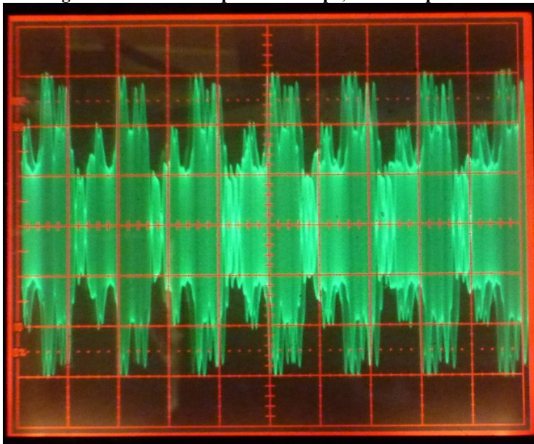
Figure 9: 100W PEP speech envelope, 6 dB compression.
