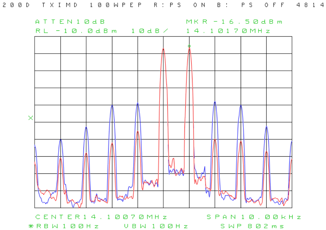
Figure 2: 2-tone TX IMD at 14.1 MHz, 100W PEP, PureSignal (PS) off & on (Test 9).
