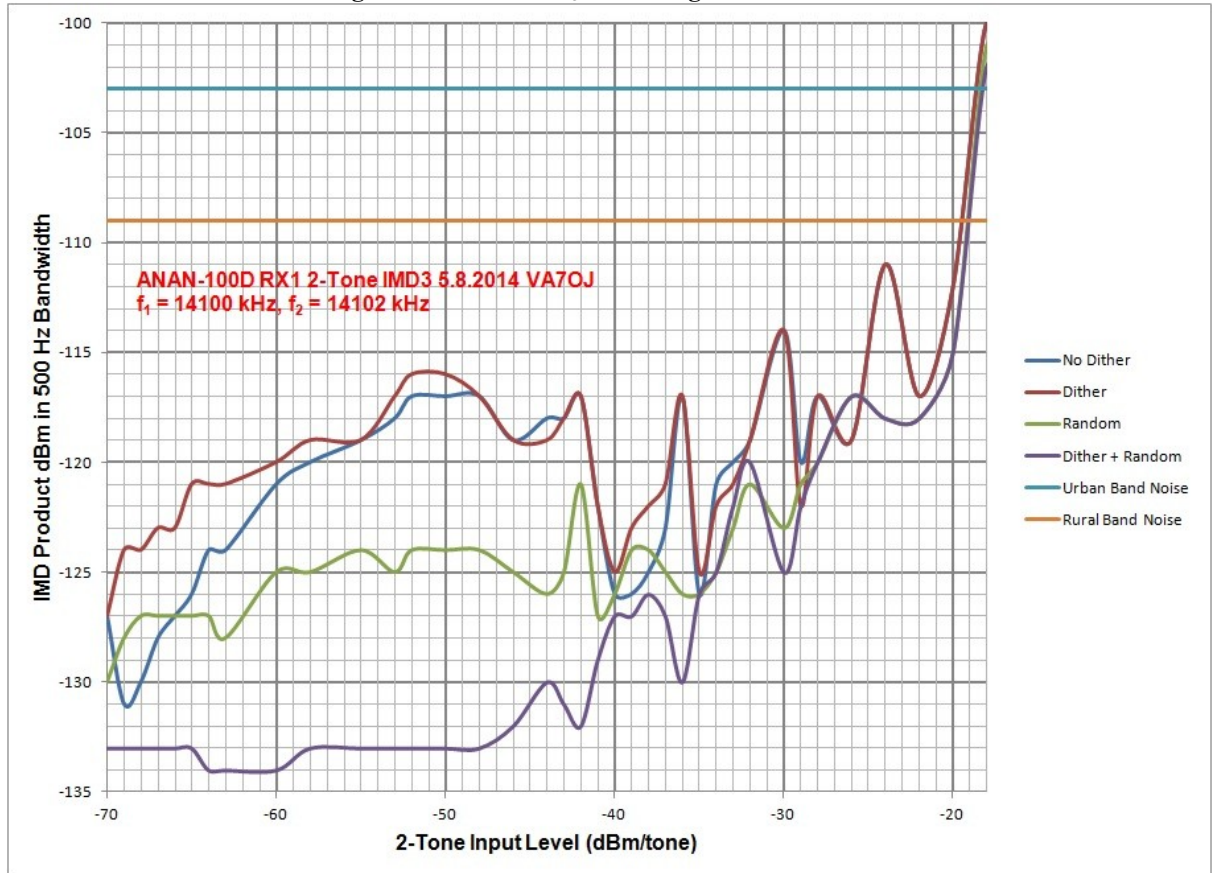
Figure 5: 2-tone IMD_3 vs. test signal level. R
