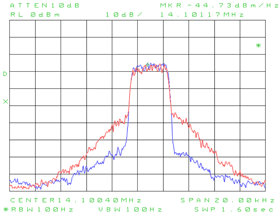
Figure 4: White Noise IMD at 14.1 MHz, 100W PEP, PureSignal (PS) off & on (Test 9a).
