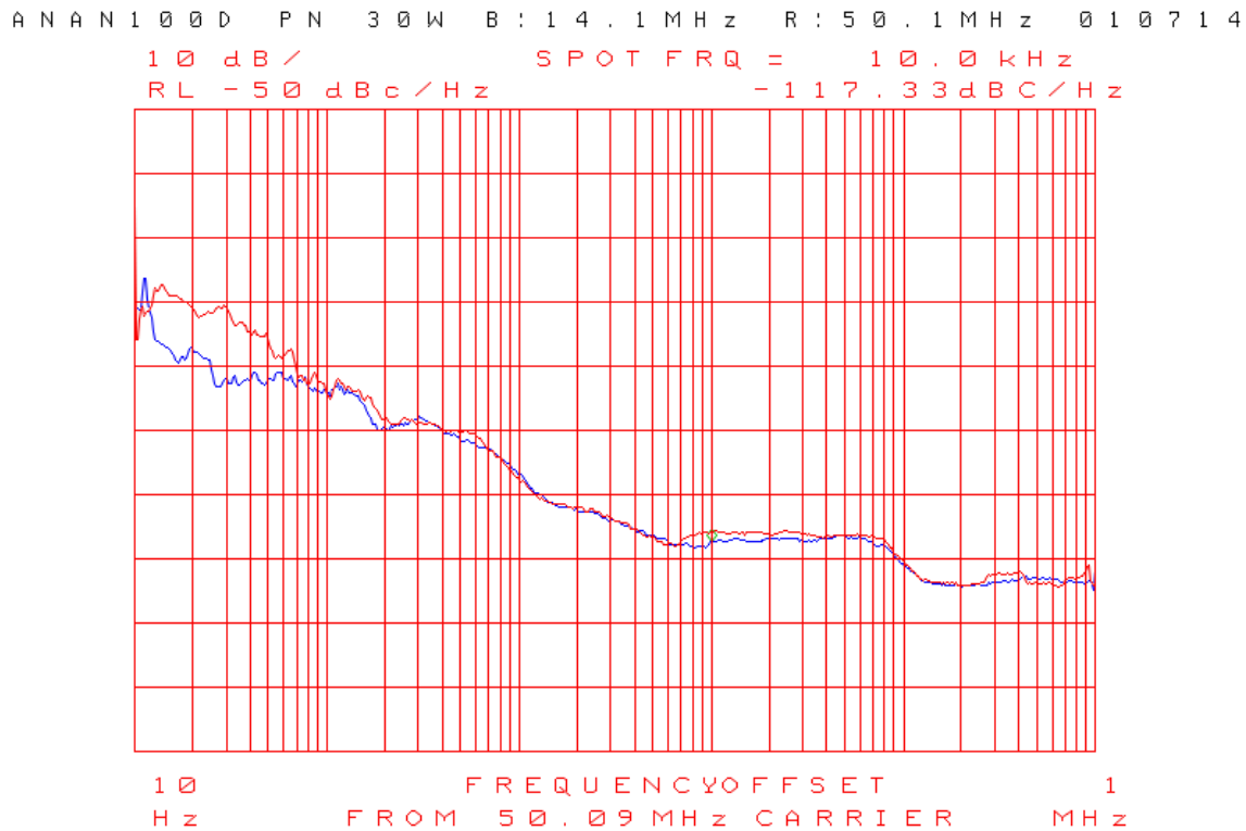
Figure 20b: Composite noise at 50.1 and 14.1MHz, 30W.
