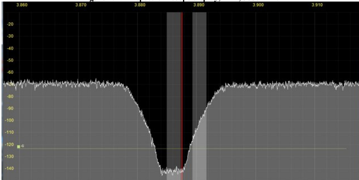
Figure 7: NPR spectrum scope display, RX1, 3886 kHz.
