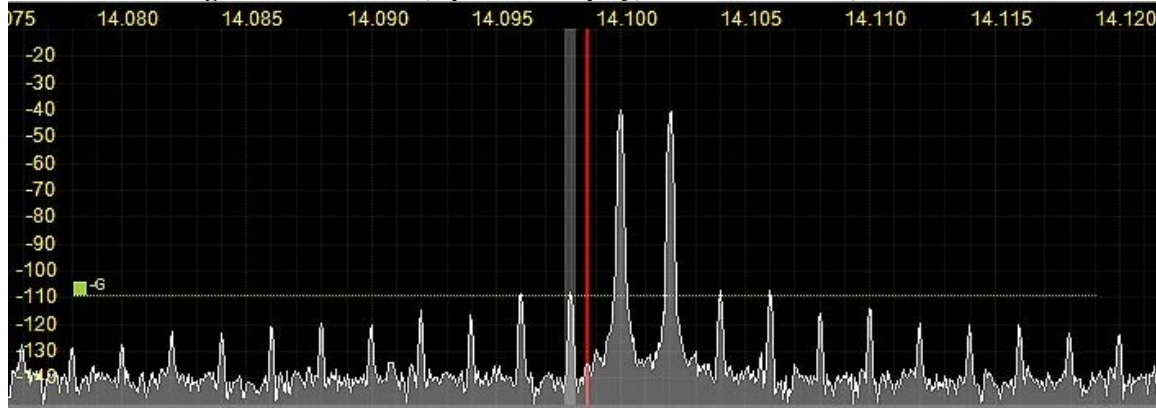
Figure 6: 2-tone IMD 3 spectrum display, P i = -40 dBm/tone, dither off.
