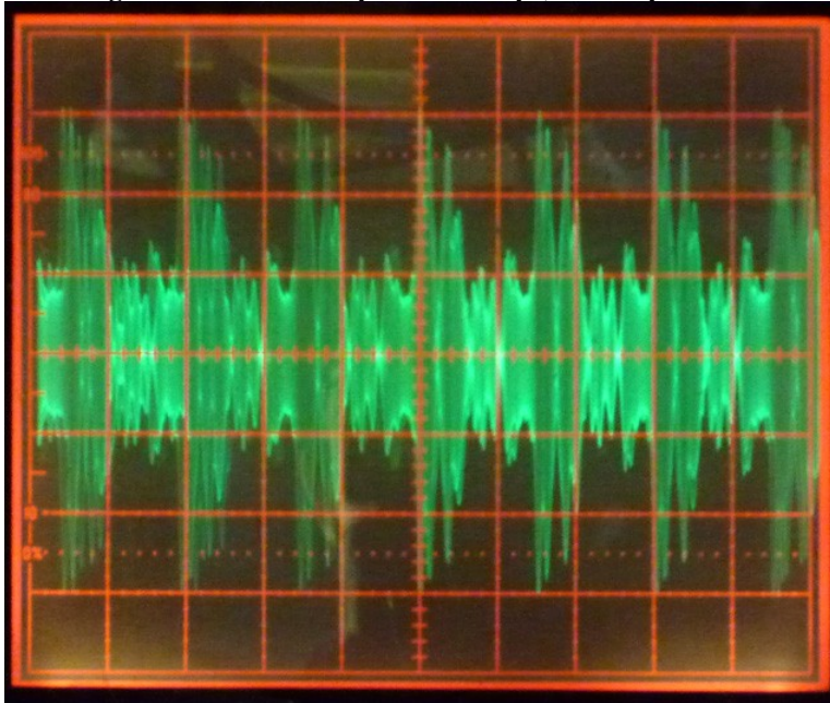
Figure 9: 100W PEP speech envelope, 6 dB compression.
