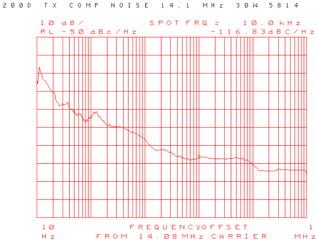
Figure 5: TX composite noise at 14.1 and 3.6 MHz, 30W.
