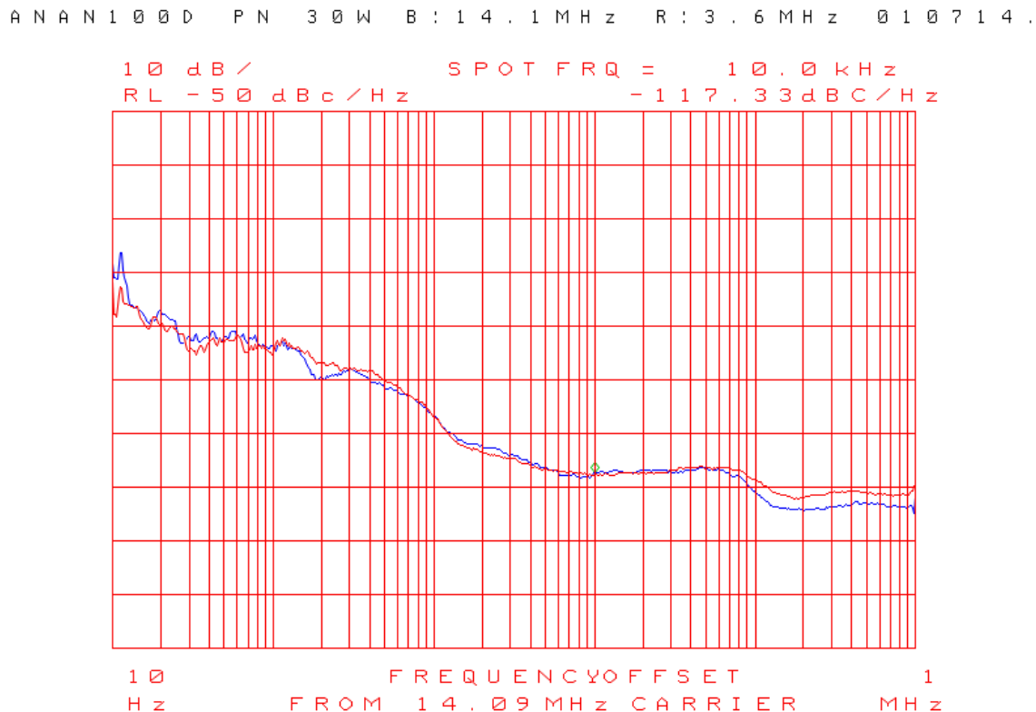
Figure 20a: Composite noise at 14.1 and 3.6 MHz, 30W.
